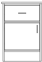
1 Drawer/1 Door 21" W, 18" D, 30" H (BAY-125)
