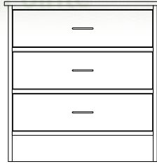
3 Drawer 30" W, 18" D, 30" H (BAY-400)
